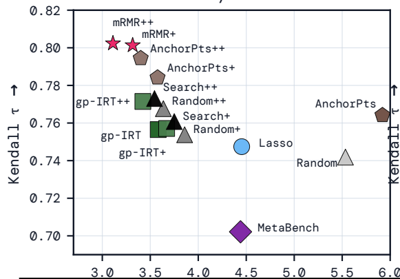
Binary Scores
