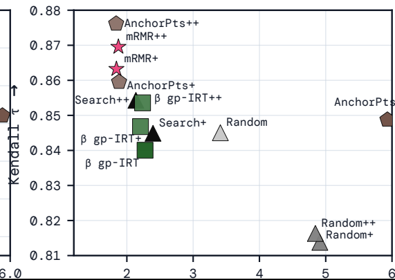
Continuous Scores
